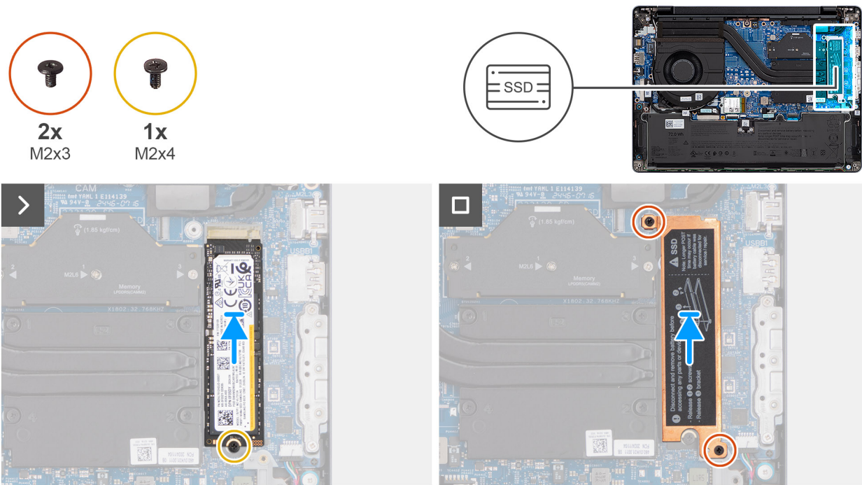
Figure 23. Installing the M.2 2280 solid state drive
