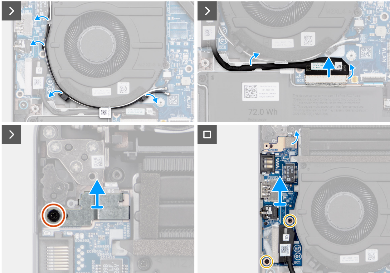
Figure 40. Removing the I/O board
