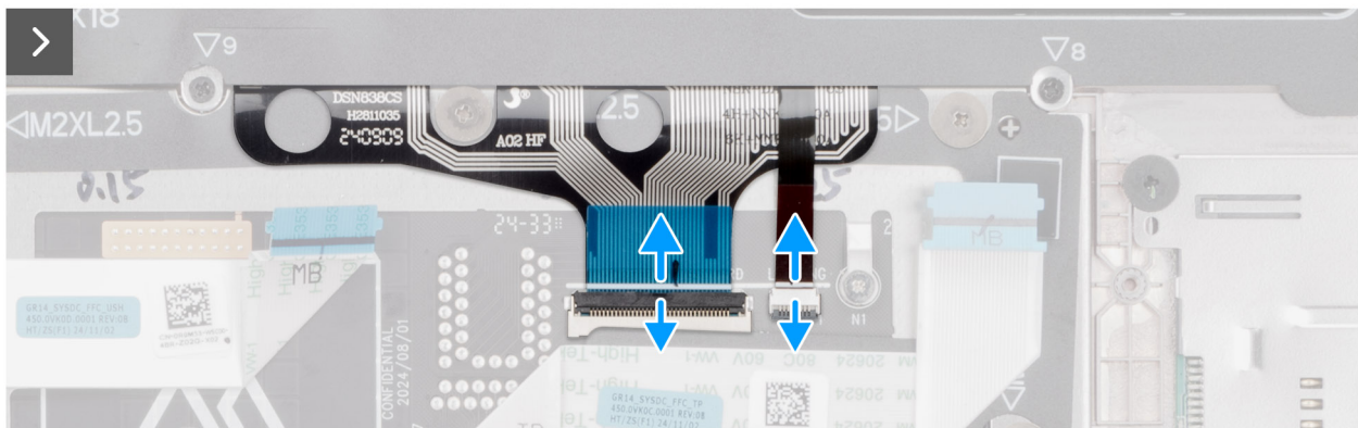
Figure 85. Removing the keyboard
