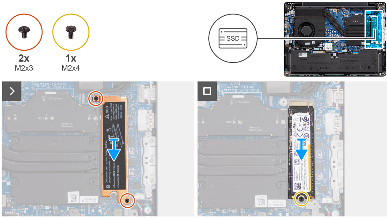
Figure 22. Removing the M.2 2280 solid state drive
