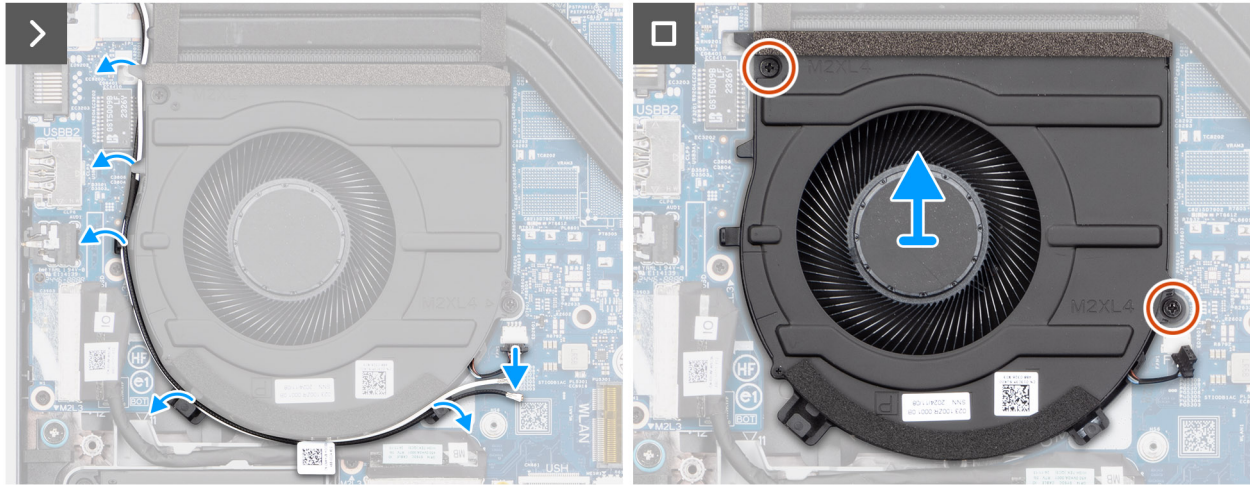
Figure 29. Removing the fan
