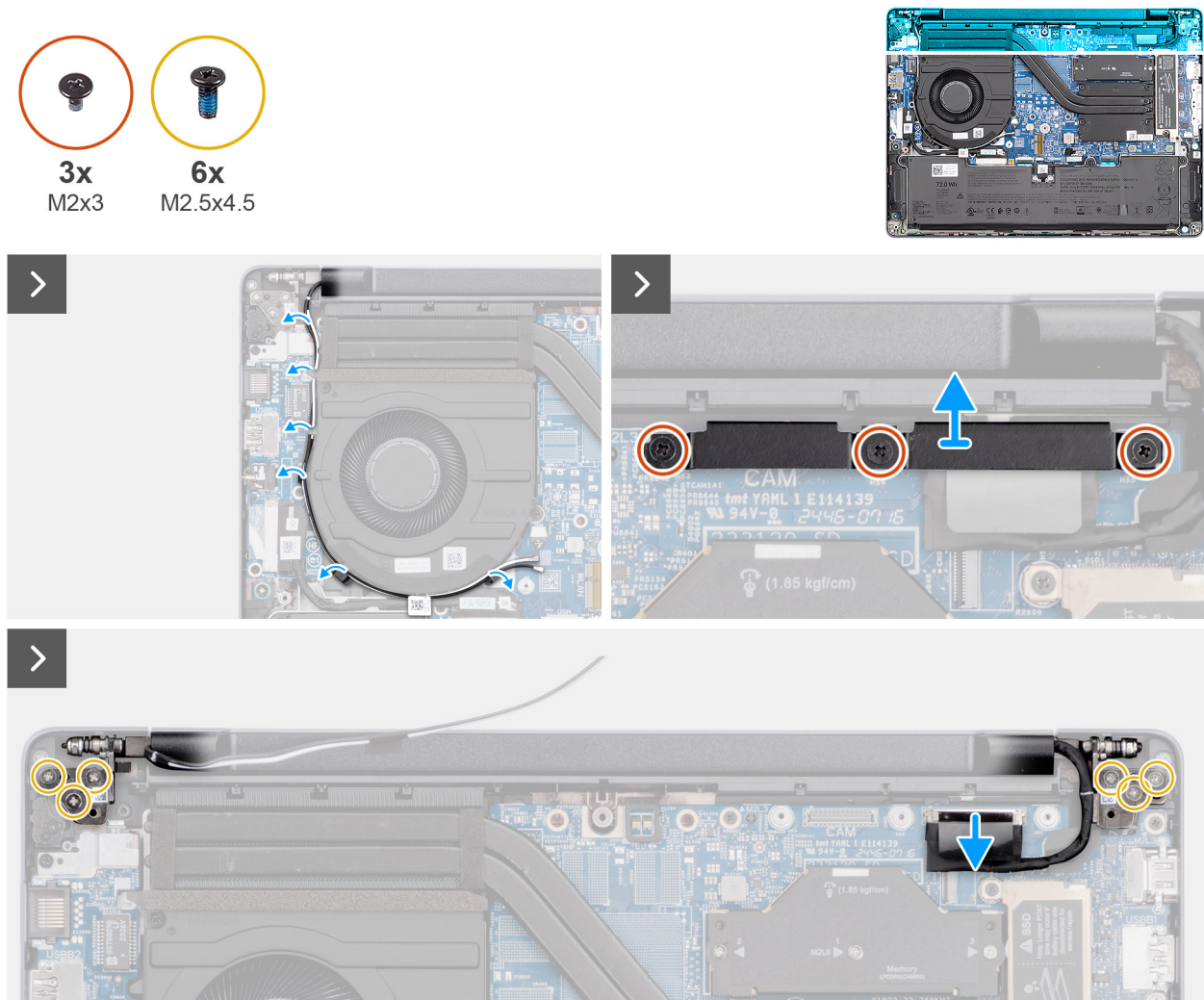
Figure 44. Removing the display assembly
