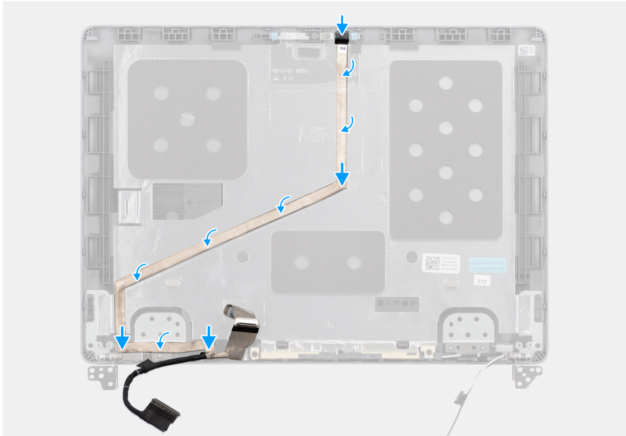
Figure 66. Installing the display cable
